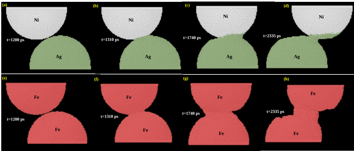
Fig. 5. Lower asperity deformation with time as the top asperity slides at a normalised interference of 0.1 in Ni-Ag and Fe-Fe metallic combination. (a) Just before asperities come into touch, (b) Atoms begin to plough at 1310 ps, (c) At the moment of 1740 ps, when asperities align vertically, (d) Asperity deformation at 2335 ps for Ni-Ag metallic combination; (e) (f), (g) and (h) are at respective times for Fe-Fe metallic combination.
