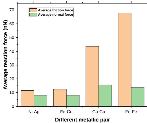
Fig. 6. Average friction and normal force for different metallic pair.
