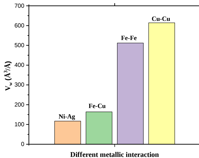
Fig. 8. Atomic wear rate for various interactions of metals at normalised interference ( \Delta/R ) of 0.1.
