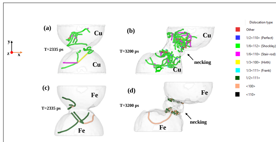
Fig. 9: Appearance of dislocation in the sliding for the interference of 0.1, (a) and (b) for interaction of Cu –Cu, (c) and (d) for interaction of Fe-Fe.
