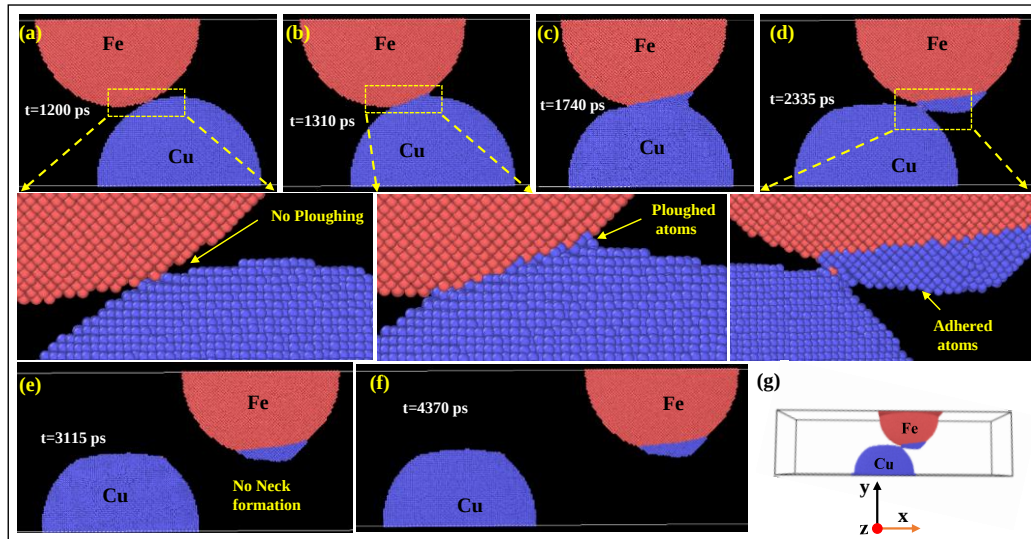
Fig. 3: Lower asperity deformation with time as the top asperity slides at a normalised interference of 0.1. (a) Just before asperities come into touch, (b) Atoms begin to plough at 1310 ps, (c) At the moment of 1740 ps, when asperities align vertically, (d) Asperity deformation at 2335 ps, (e) and (f) are front views of interacting asperities at respective times, (g) is three-dimensional perspective view.
