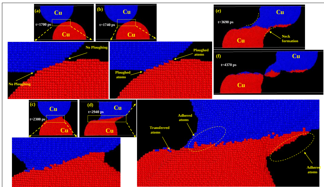
Fig. 7: Deformation in copper asperities (a) at time ( t ) = 1700ps (b) at time ( t ) = 1740 ps (c) at time ( t ) = 2300 ps (d) at time ( t ) = 2940 ps (e) at time ( t ) = 3690 ps (f) at time ( t ) = 4370 ps.
