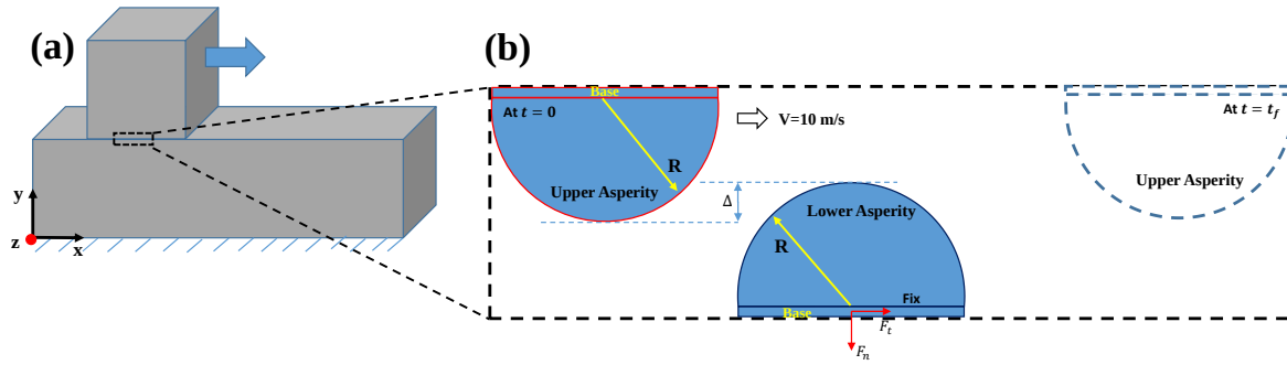
Fig. 1. (a) Schematic of a sliding contact between nanosurfaces used in NEMS/MEMS devices (b) Representation of sliding between two nano-asperities.
