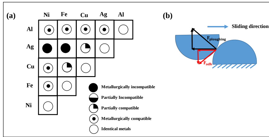
Fig. 2. (a) Metallurgically compatibility chart (b) Schematic of reaction forces in sliding contact between two hemispherical asperities.
